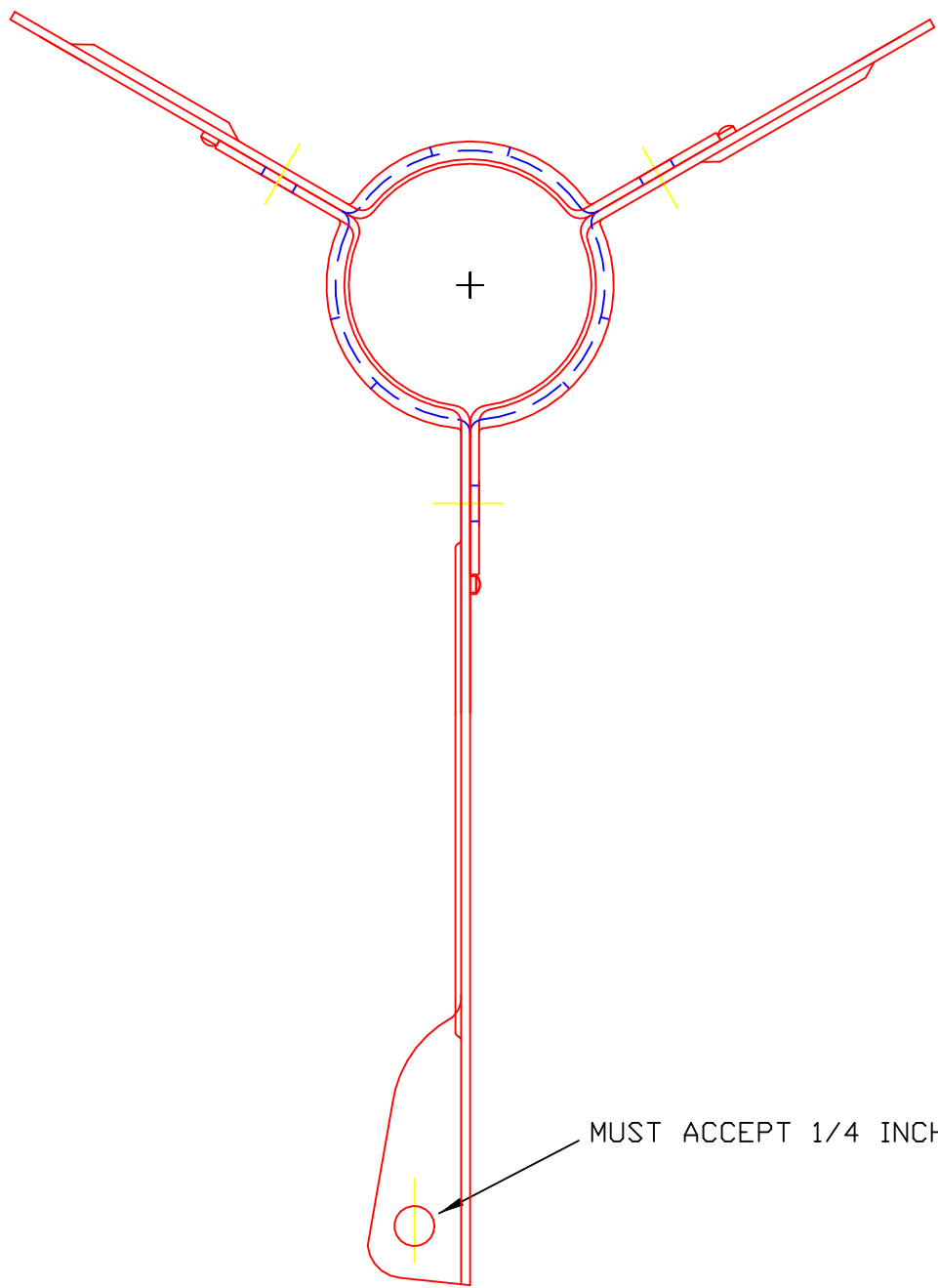
Triangle Mfg Co. "TA" Style Tri-Arm Example
